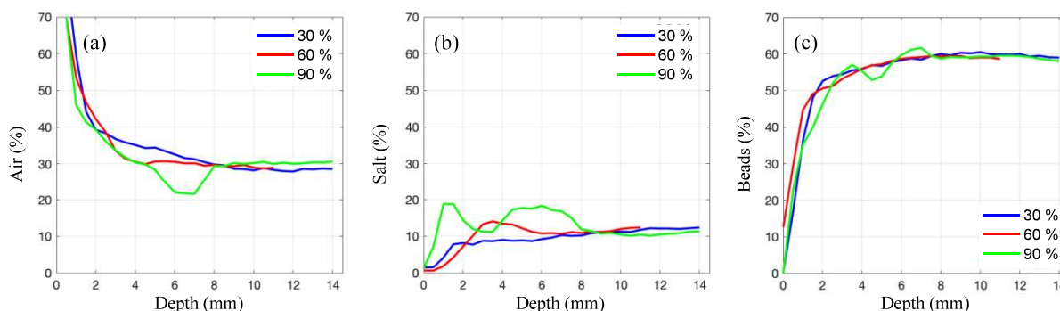
Figure 4: The fractions of voxels categorized as (a) air, (b) salt and (c) glass beads were measured from the segmented data, and horizontal slices extracted at different depths from the evaporating surface. Results are shown for specimens initially filled with sodium sulfate solutions at 30% (blue), 60% (red) and 90% (green) of saturation.
